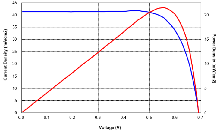
Current-Voltage Characteristics
