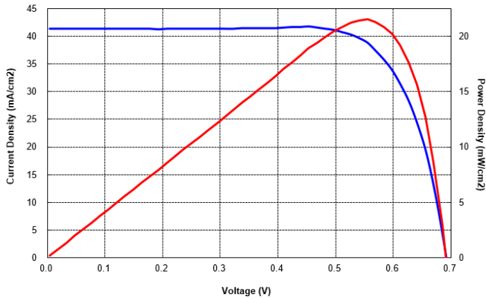
Current-Voltage Characteristics
