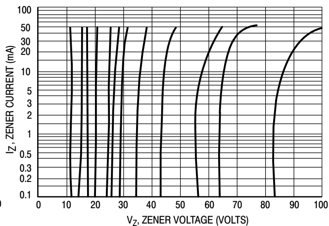
Figure 8. V_Z = 12 to 82 Volts
