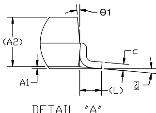
DETAIL "A"
