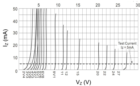
Figure 2. Breakdown Characteristics
