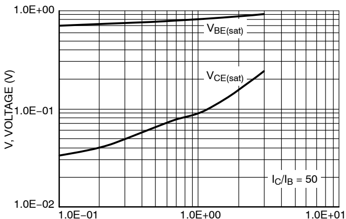
Figure 5. "ON" Voltages
