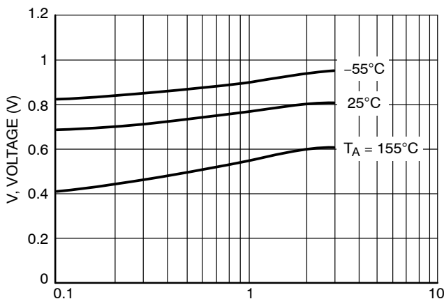
Figure 6. V_{BE(on)} Voltage
