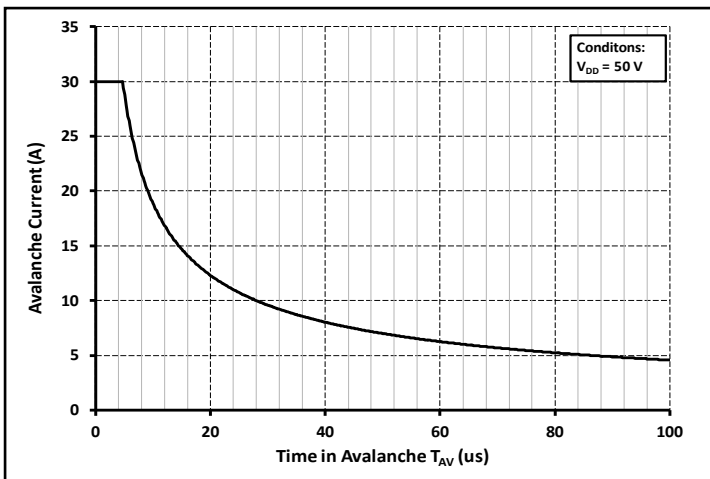
Figure 29. Single Avalanche SOA curve
