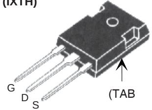
TO-247 (IXTH)
