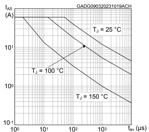
Figure 10. Avalanche characteristics
