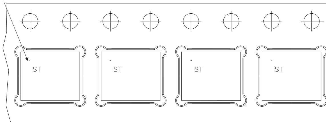
Figure 21. PowerFLAT 5x6 reel
