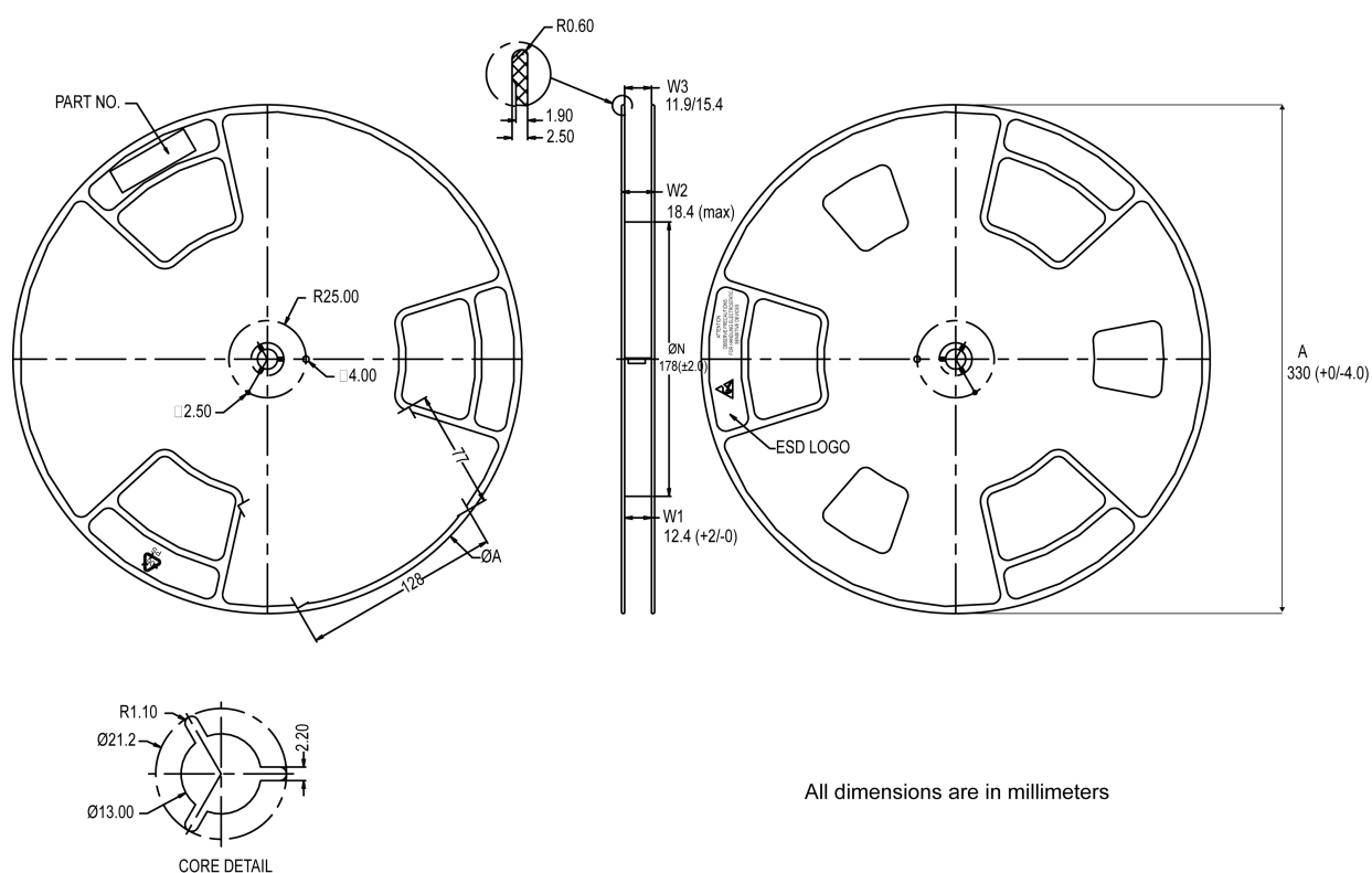
Figure 21. PowerFLAT 5x6 reel
