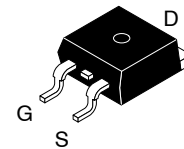
D2PAK-3 (TO-263, 3-LEAD) CASE 418AJ
