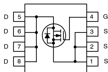
N-Channel MOSFET
