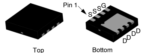
WDFN8 3.3x3.3, 0.65P CASE 511DQ (Option A) FDMC4435BZ-F127-L701
