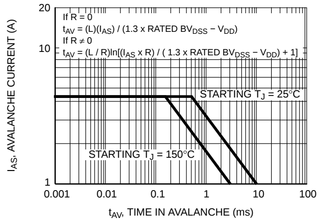
Figure 8. Unclassified Inductive Switching Capability
