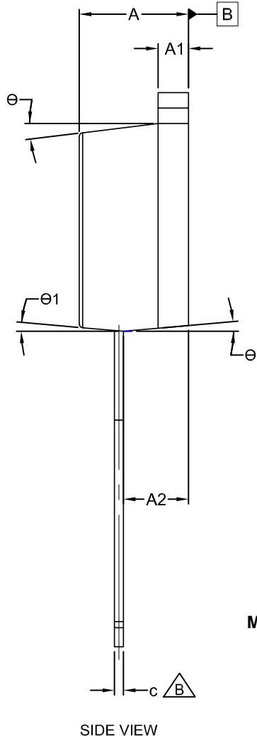
SIDE VIEW
