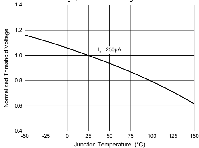
Fig. 6 - Threshold Voltage
