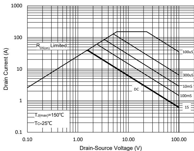
Fig.12 Safe Operation Area
