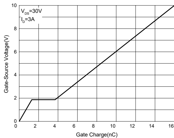
Fig. 6 - Gate Charge
