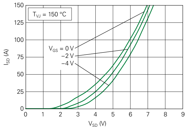
Fig. 12. Typical Reverse Conduction Characteristics ( T_{VJ} = 150^{\circ} C)
