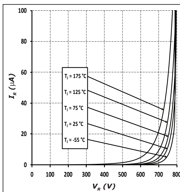
Figure 2. Reverse Characteristics
