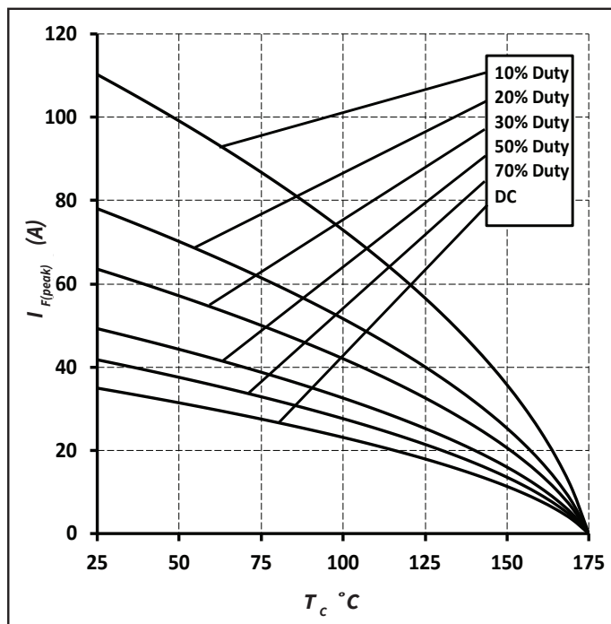
Figure 3. Current Derating
