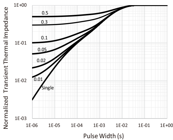
Figure 8: Transient Thermal Impedance (Per Component)
