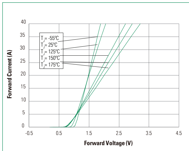
Figure 1: Typical Foward Characteristics
