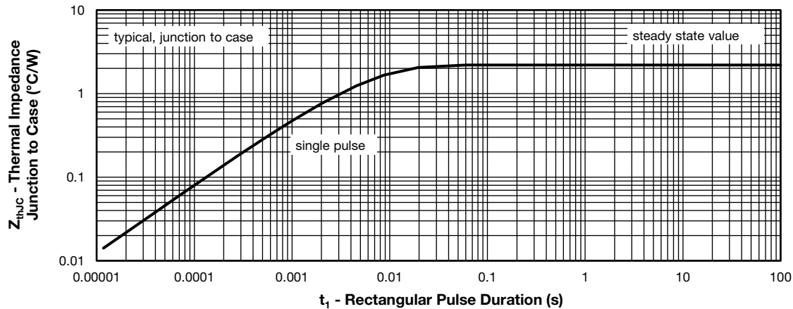
Fig. 9 - Transient Thermal Impedance, Junction to Case
