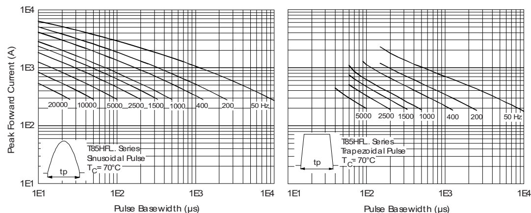
Fig. 43 - Frequency Characteristics
