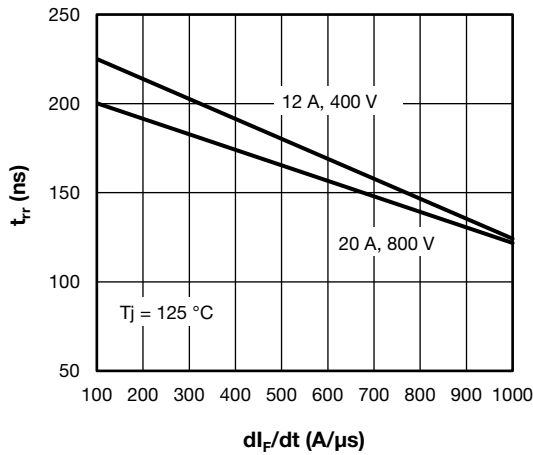
Fig. 7 - Typical Reverse Recovery Time vs. di/dt
