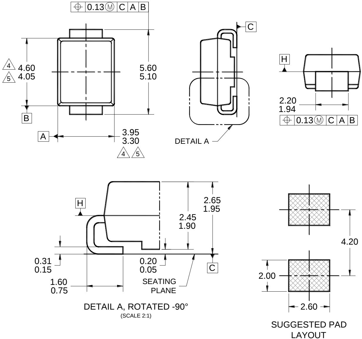
DO-214AA (SMB)
