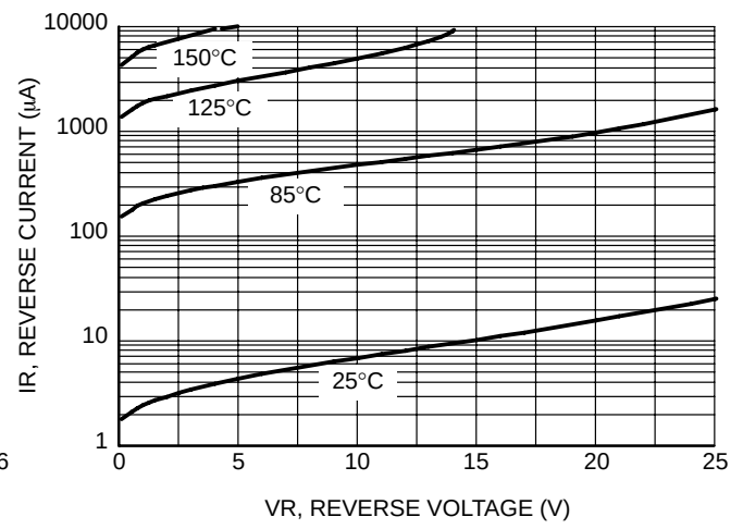
Figure 2. Leakage Current
