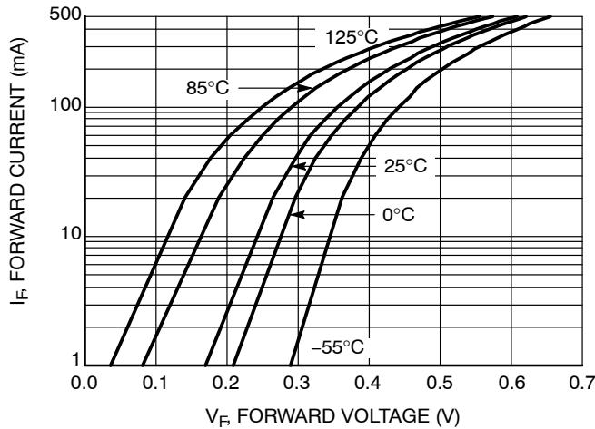
Figure 3. Forward Voltage
