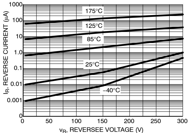
Figure 3. Maximum Reverse Voltage
