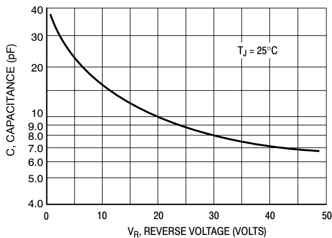
Figure 10. Typical Capacitance
