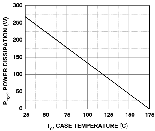
Figure 5. Power Derating
