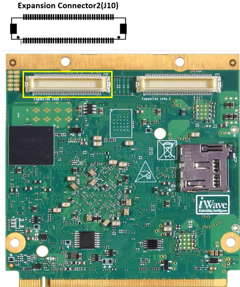
Figure 9: Expansion Connector2
