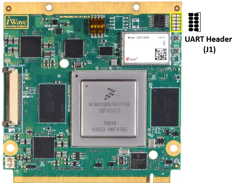
Figure 11: UART Header
