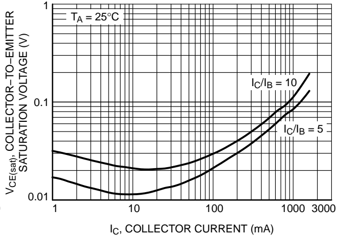
Figure 9. VCE(sat) – IC
