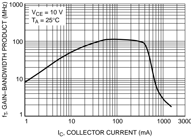
Figure 10. fT – IC
