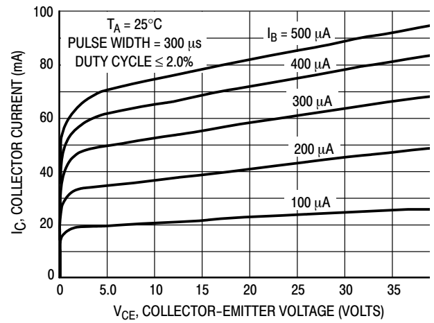
Figure 10. Collector Characteristics
