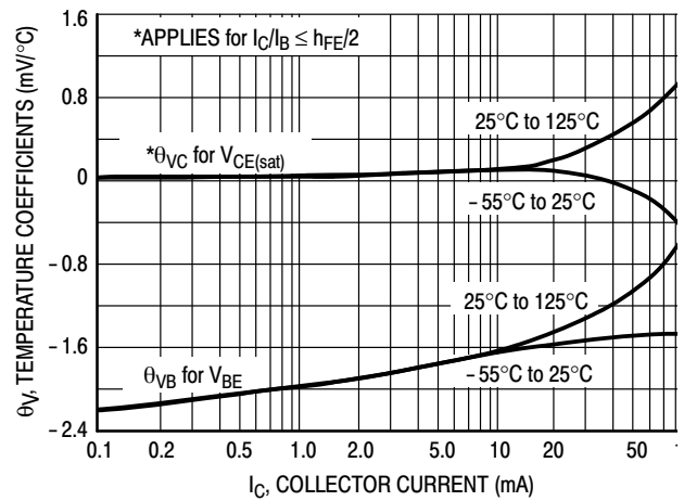
Figure 12. Temperature Coefficients
