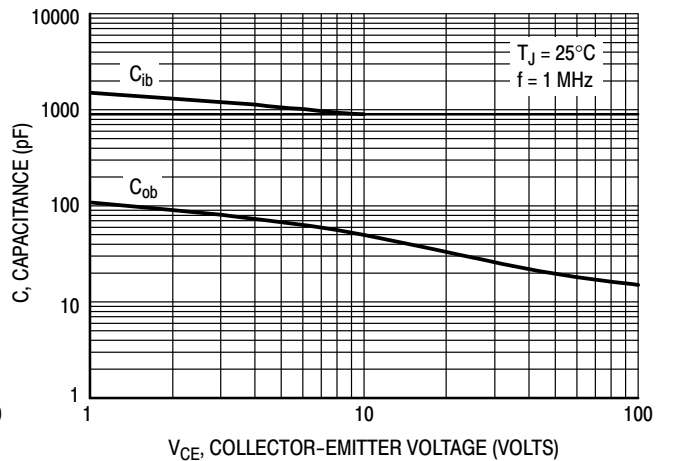
Figure 6. Capacitance
