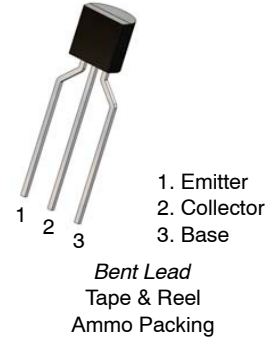
TO-92 3 4.83x4.76 LEADFORMED CASE 135AR
