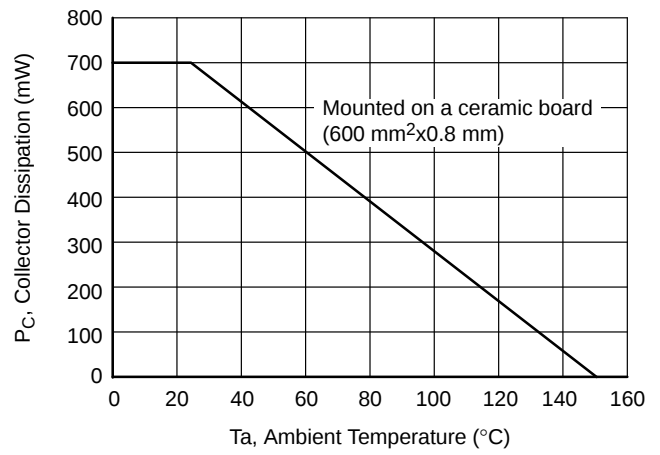
Figure 11. P_C - T_a
