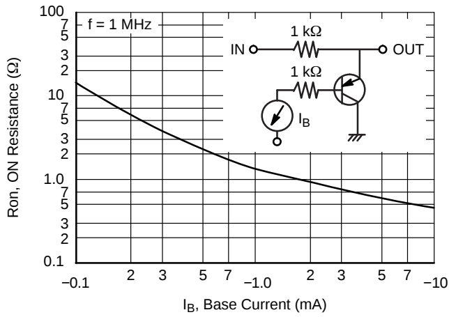
Figure 10. R_{on} - I_B
