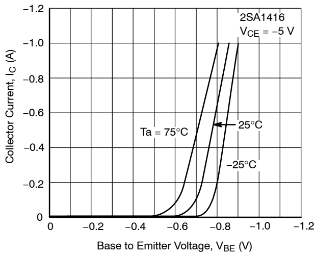
Figure 5. I_C - V_{BE}
