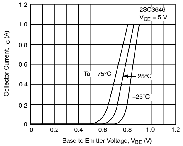
Figure 6. I_C - V_{BE}
