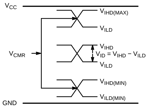
Figure 8. V_{CM} Diagram
