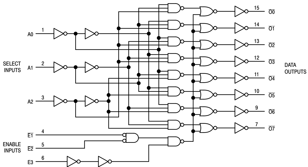
Figure 1. Logic Diagram
