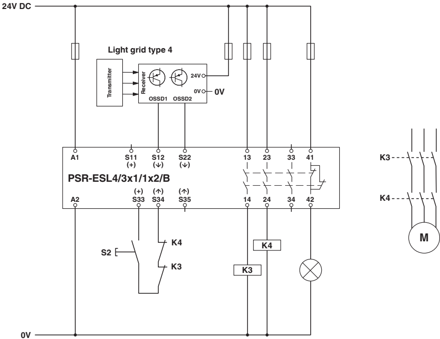
Circuit diagram
