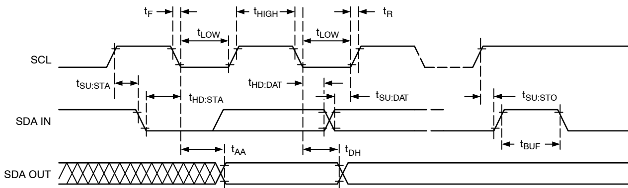
Figure 8. Bus Timing
