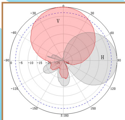
Radiation Pattern 915 MHz
