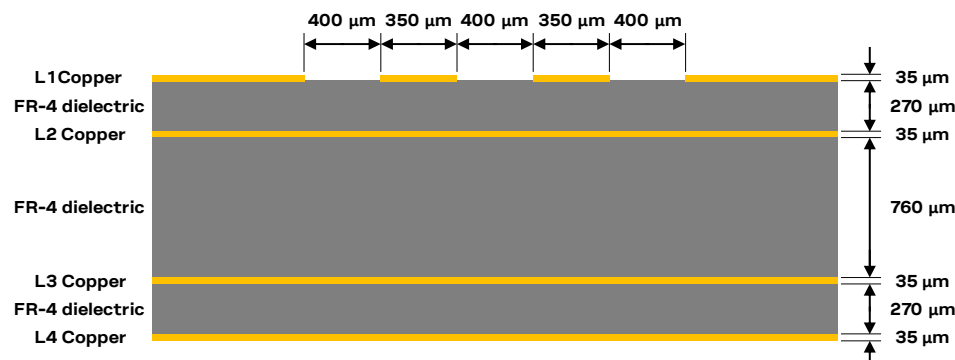
Figure 66: Example of USB line design, with Z_0 close to 90 \Omega and Z_{CM} close to 30 \Omega , for the described 4-layer board layout
