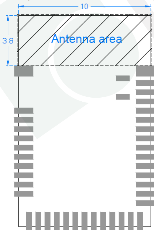
Top View (Unit: mm)
