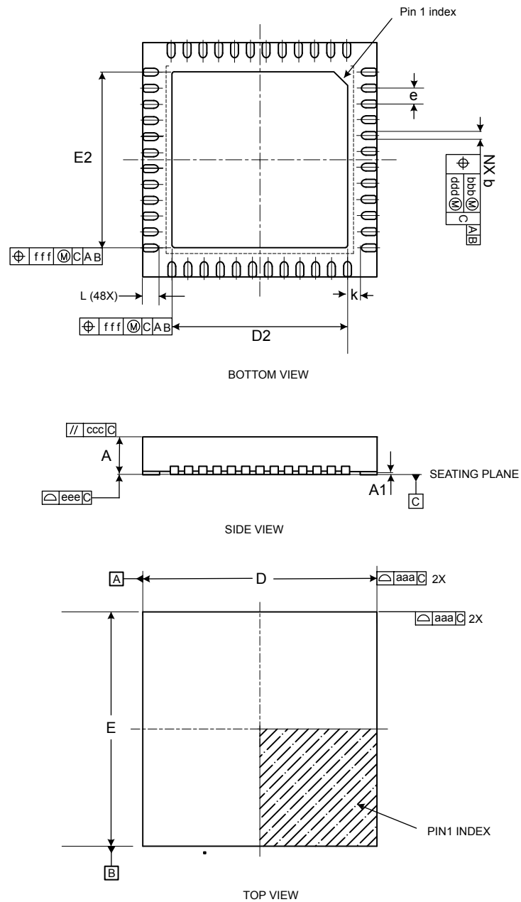
Figure 19. VFQFPN48 - Outline
