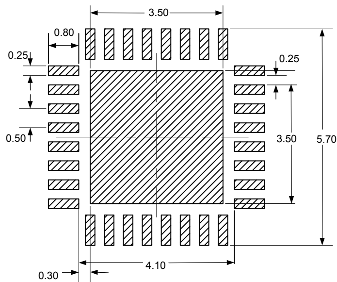
Figure 22. VFQFPN32 - Footprint example
