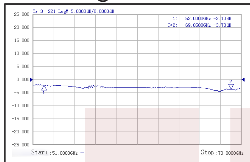
Insertion Loss@+25°C
