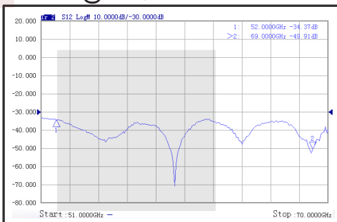
Isolation@+25°C
