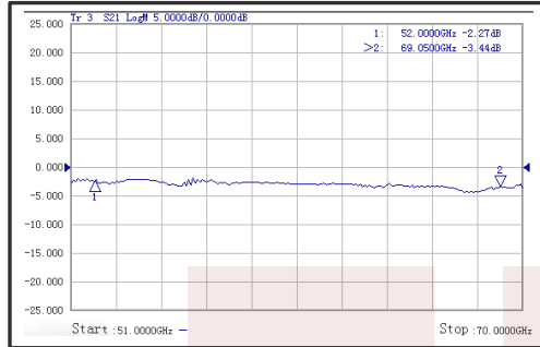
Insertion Loss@-40°C
