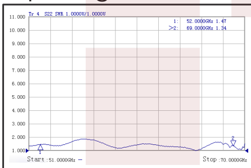
Output VSWR@+85°C
