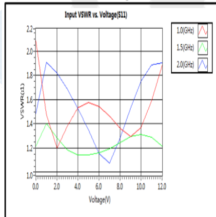
Input VSWR vs. Voltage
