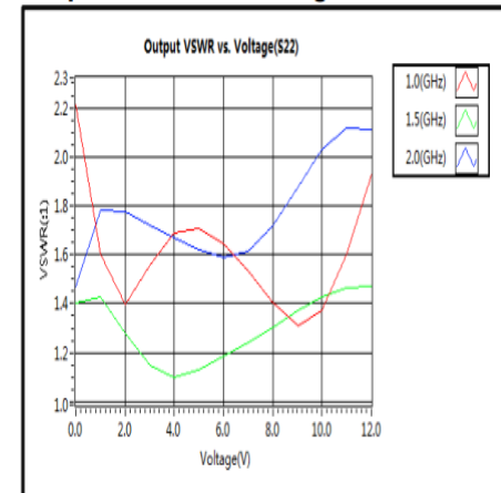
Output VSWR vs. Voltage
