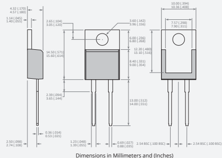
TO-220 2-Lead
