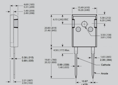
TO-247 2-Lead
