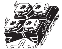
SOT-227[J] Antiparallel Configuration (Isolated Base)
