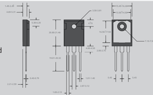
TO-247-3-Lead
