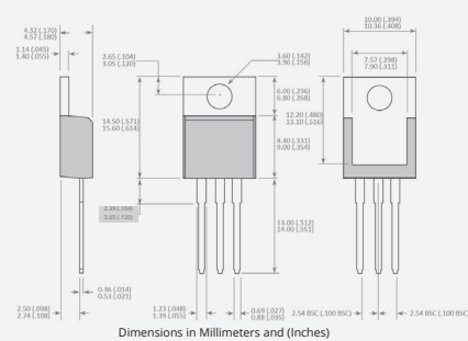
TO-220 3-Lead
