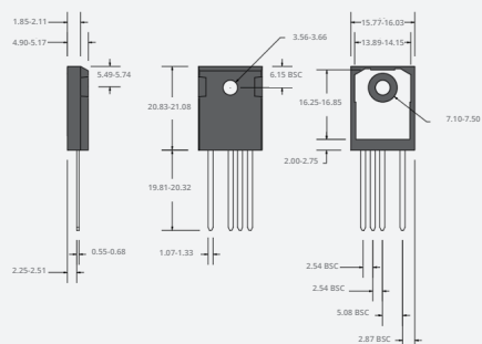
TO-247-4-Lead
