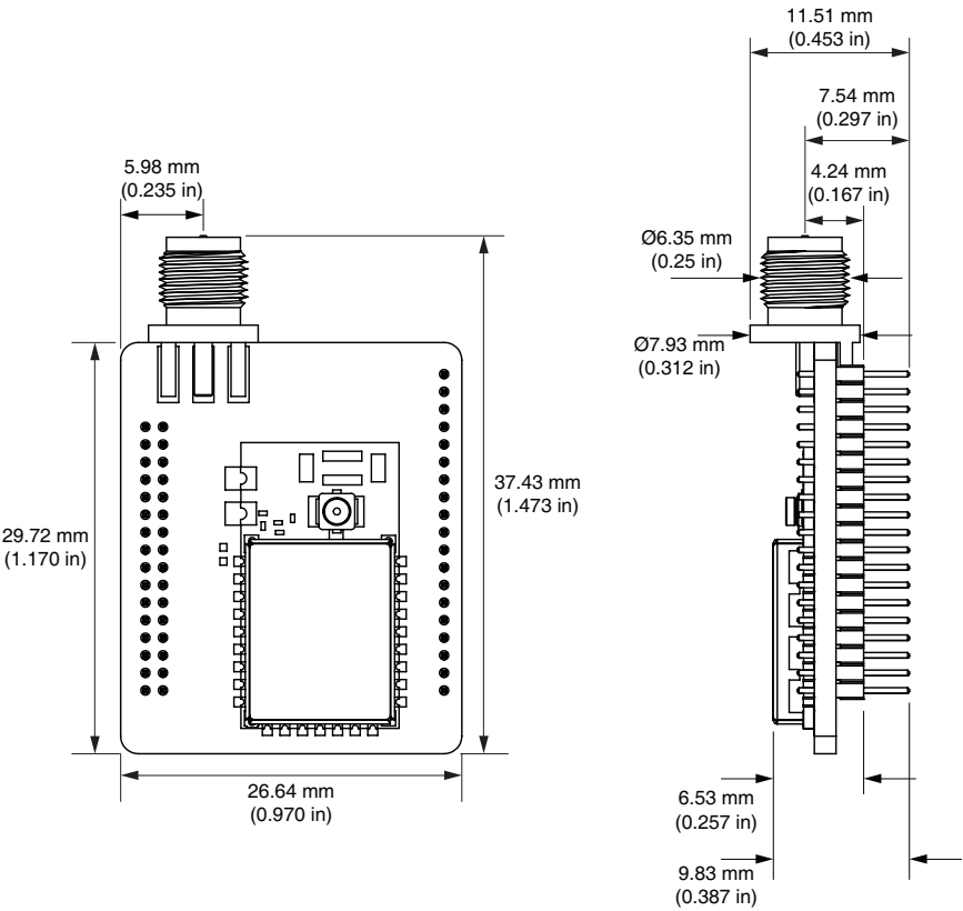
Figure 13: EVM-fff-PRC-CAS Dimensions
