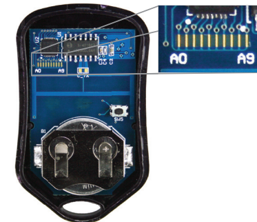
Figure 6: Address Traces
